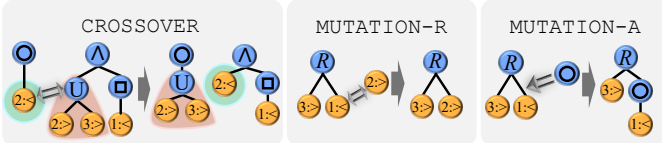
Fig. 3. The illustration of the operations in the offspring generation. For each pTLTL tree in the figure, the blue nodes represent logical operators, and the orange nodes represent pAP nodes. The labels of the pAP node indicate the semantics of pAP; for example, the label '2:<' refers to s^{(2)} < \theta for an undetermined parameter \theta .
