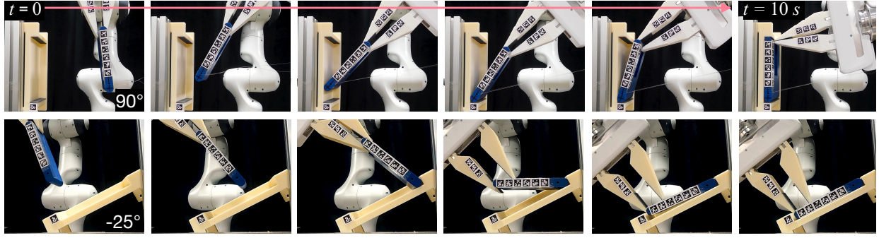
Fig. 6. Demonstration of ILCL's constraint transfer capability in the peg-in-shallow-hole environments. By creating real-world environments with holes tilted at 90^\circ , 60^\circ , and -25^\circ , we enable the Panda gripper to find a constrained policy using the learned constraints and reproduce a demonstration-like robust insertion with stable contact in each unseen environment. Demonstration videos are available in the supplementary materials including 60^\circ tilted hole insertion.
